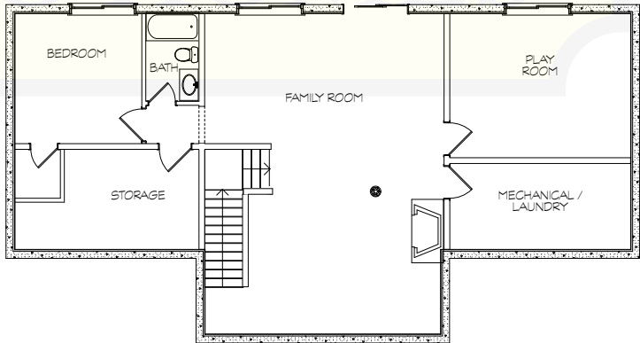
BASEMENT
